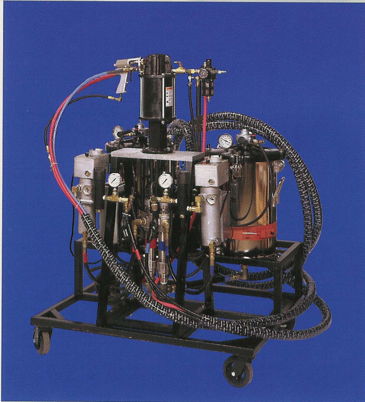
CPE-600 with 10 Gallon Stainless Steel Tanks
